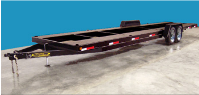
Model C32 Tag-a-long 2 Car Hauler 14,000 GVWR
